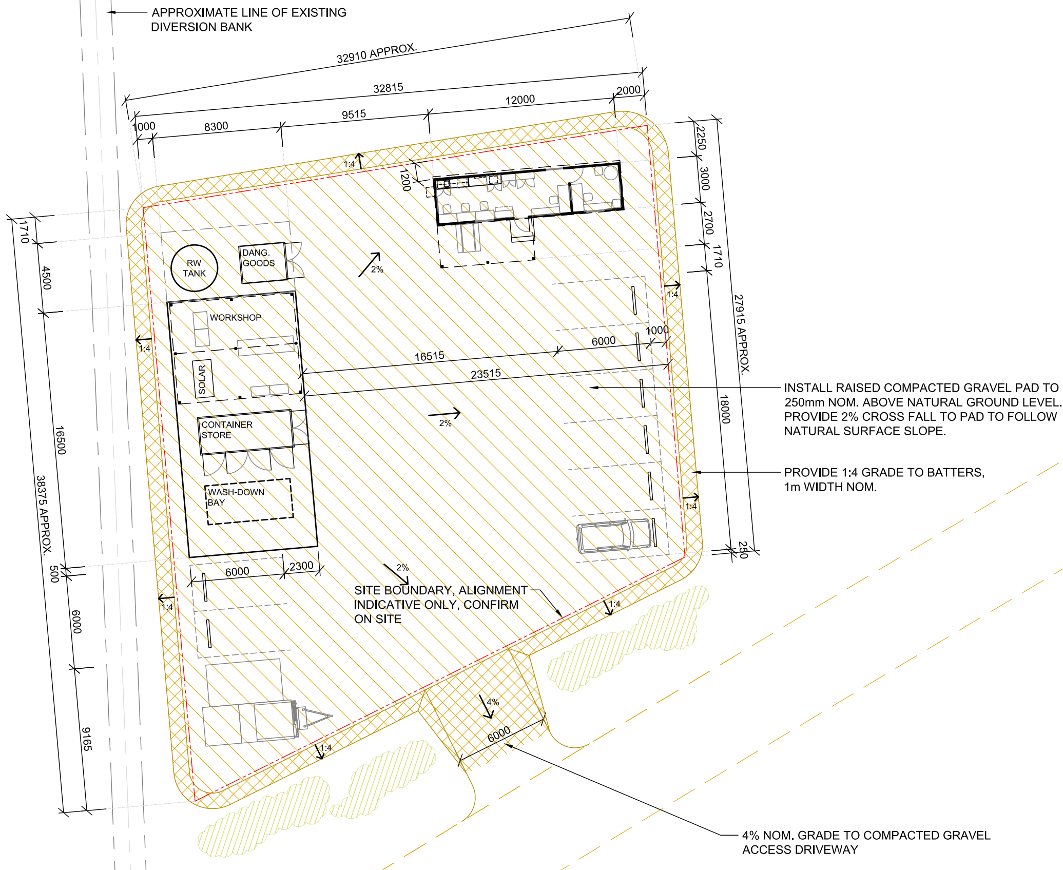
SITE SETOUT AND GRADING SCALE - 1:250
