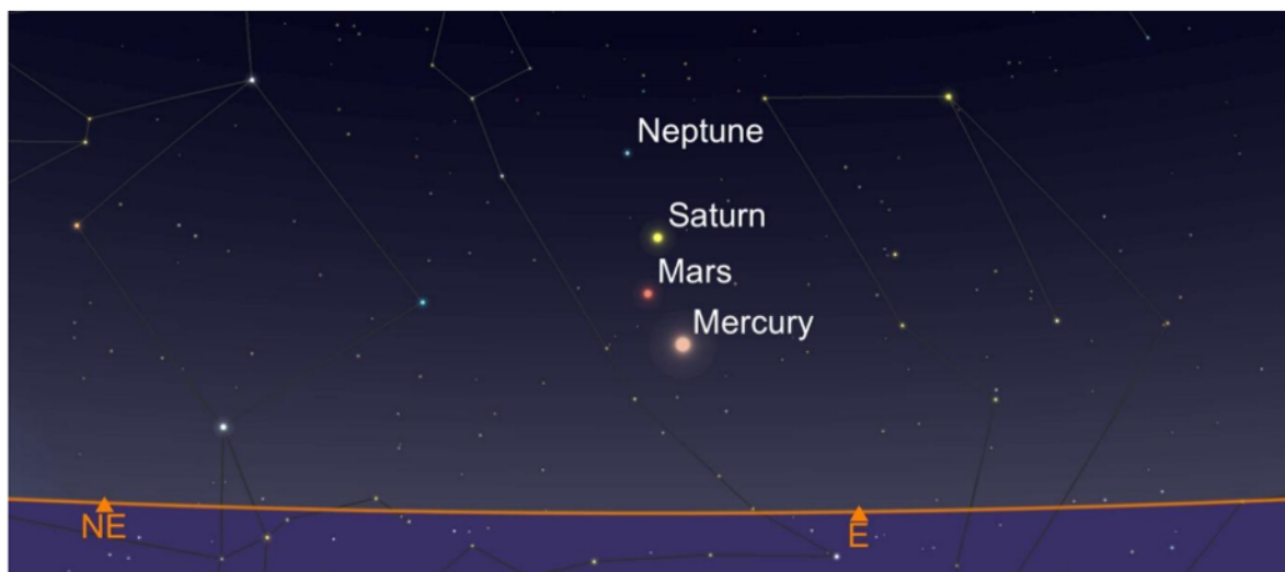
An alignment of planets will watch over dawn services on Anzac Day. Image provided by SkySafari, a Simulation Curriculum Company, All rights reserved www.simulationcurriculum.com .
