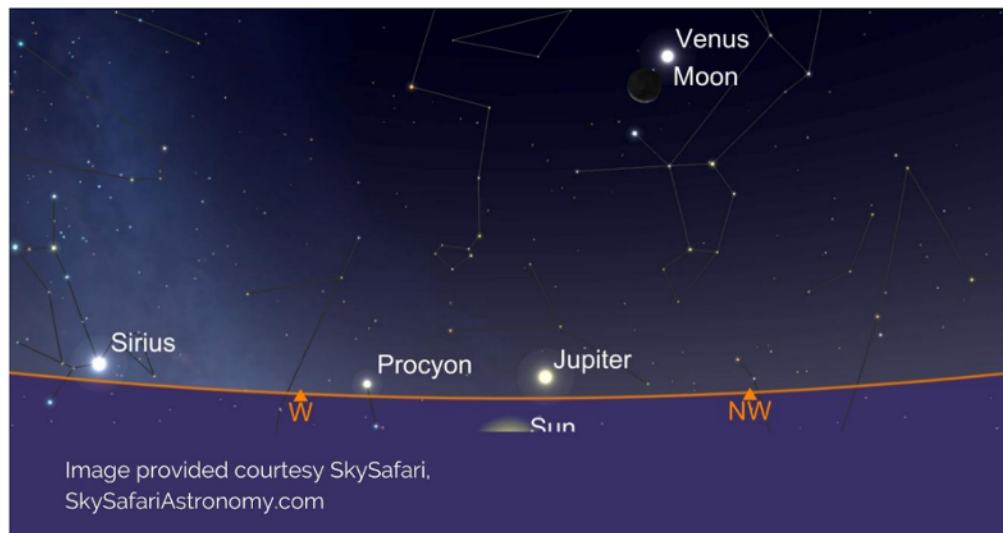
Dazzled by the Moon and Venus at 6pm on 17th June. Image provided by SkySafari, a Simulation Curriculum Company, All rights reserved www.simulationcurriculum.com .
